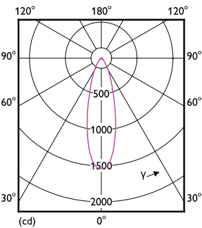
Light Distribution Diagram - 8PAR16/LED/830/F25/DIM/G/120V 6/3FB
