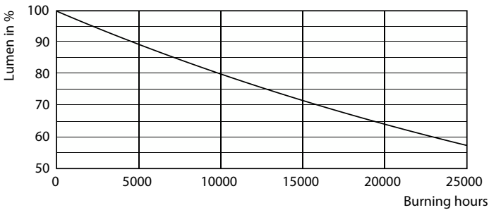
Lumen Maintenance Diagram - 8PAR16/LED/830/F25/DIM/G/120V 6/3FB
