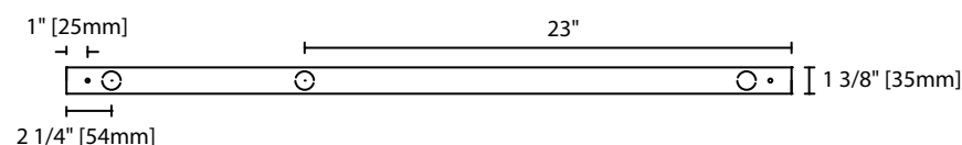
ST1 T5 Base View *
