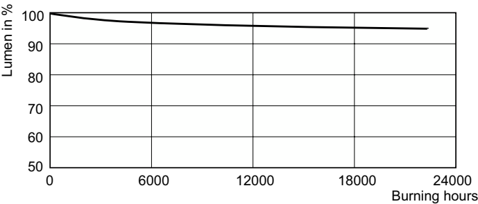
Lumen Maintenance Diagram - SOX 55W BY22d 1SL
