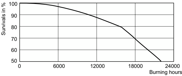
Life Expectancy Diagram - SOX 55W BY22d 1SL
