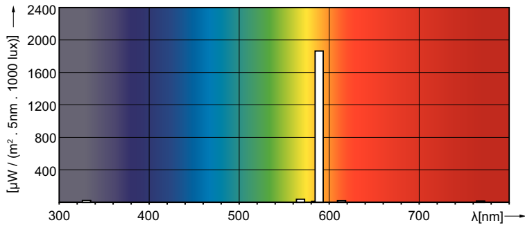
Spectral Power Distribution Colour - SOX 55W BY22d 1SL
