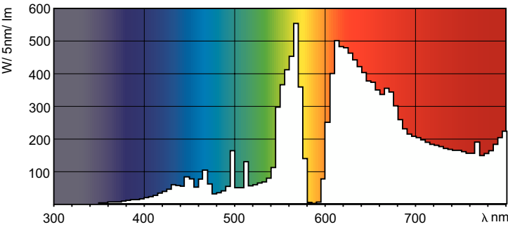
Spectral Power Distribution Colour - SDW-TG 100W/T6/825 12PK
