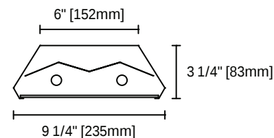
HB 2 Lamp Cross Section View
