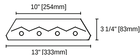
HB 4 Lamp Cross Section View
