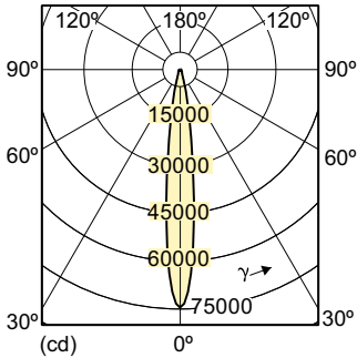
CDM-R Elite 70W /930 PAR30L 10D
