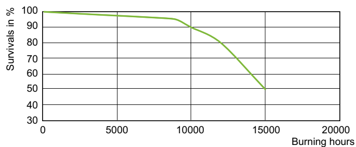
CDM-R Elite 35W Life Expectancy /930 PAR20
