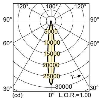
CDM-R Elite 35W /930 PAR20 10D
