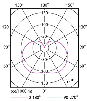
Light Distribution Diagram - 65HB/LED/850/ND FB 4/1
