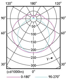
Light Distribution Diagram - 16.5PL-L/COR/22-830/IF22/P/4P/DIM 10/1
