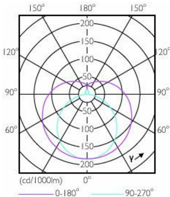
Light Distribution Diagram - 8T5HE/22-840/IF10/G/DIM 10/1
