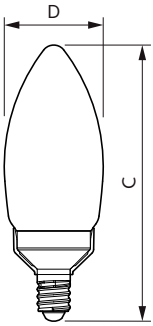
Candle B11 120V 4.5-40W 300lm 2200-2700K
