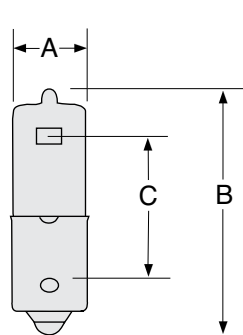
BA9s
